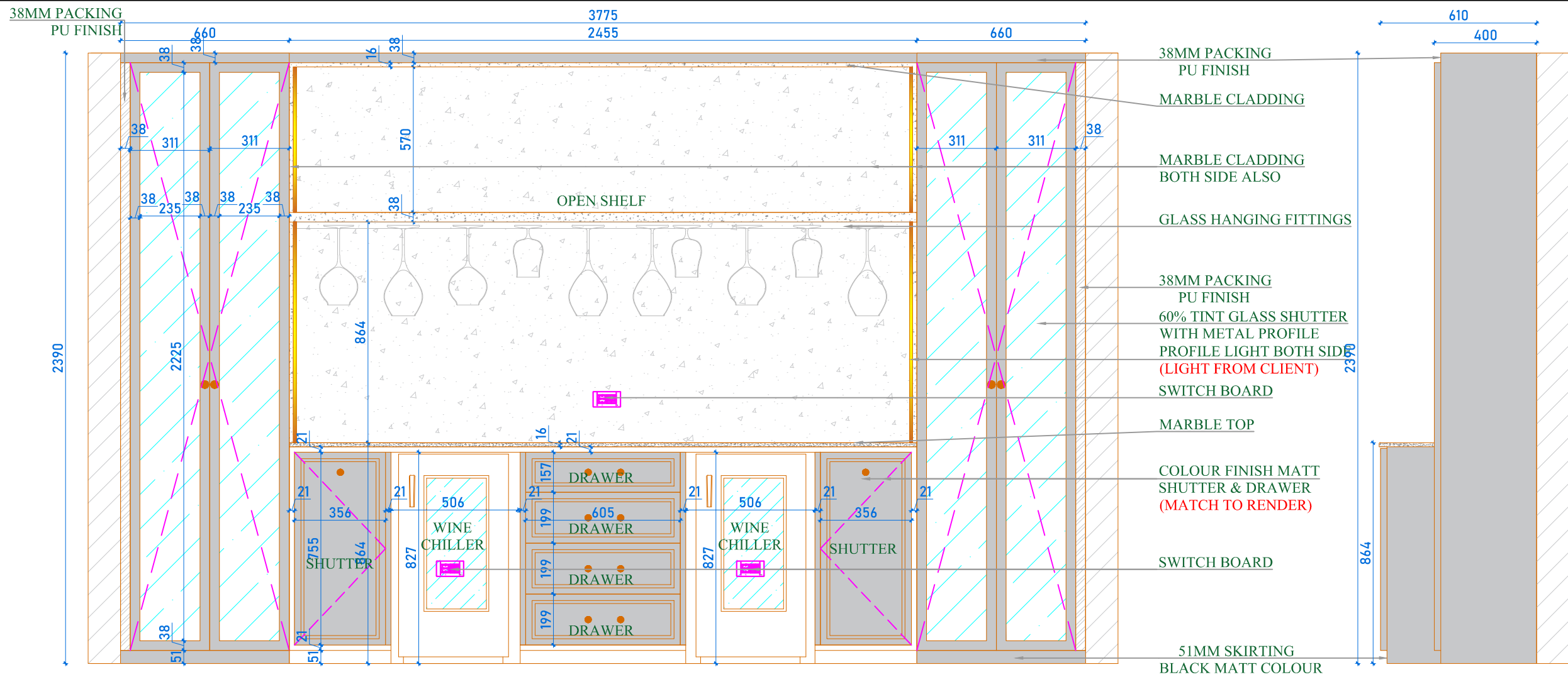
FRONT ELEVATION
